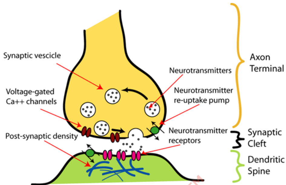
Fig. 5. Chemical synapses
