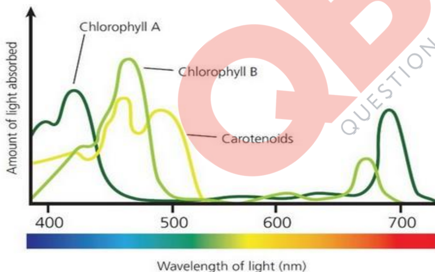
The absorption spectra of extracted chlorophyll and carotenoids. The primary light harvesting chlorophylls absorb light in the blue and red regions. Carotenoids absorb in the blue and green regions.
