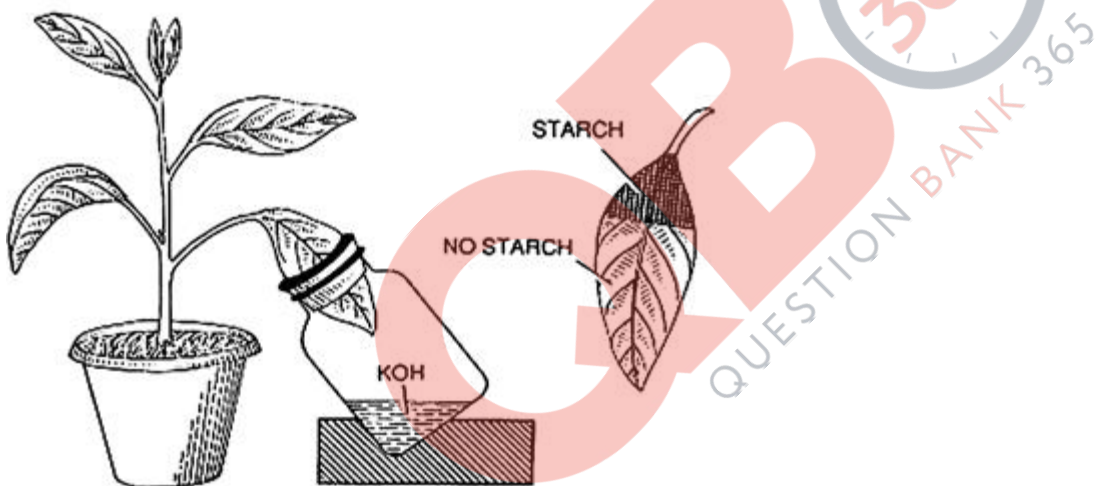
Fig 5.27. Mohl's experiment.
